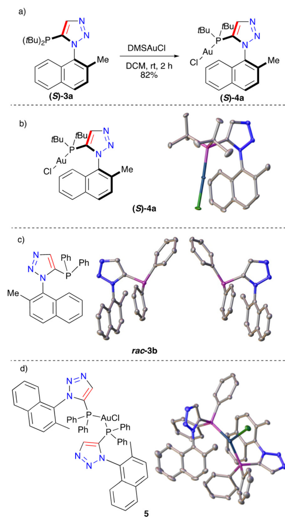
Fig. 3 (a) Synthesis of a single enantiomer gold(i) chloride complex (b) single-crystal X-ray diffraction structure of (S) - 4a . Ellipsoids are drawn at the 50% probability level. A molecule of \text{DCM} has been omitted for clarity. Hydrogen atoms omitted for clarity. (c) Molecules from the crystal structure of rac - 3b with ellipsoids drawn at the 50% probability level. Symmetry codes used to generate the equivalent atoms: (i) x, y, z , (ii) 1 - x, 1 - y, 1 - z . Hydrogen atoms omitted for clarity. (d) Single-crystal X-ray diffraction structure of homo-chiral complex 5 . Ellipsoids are drawn at the 50% probability level. A molecule of \text{DCM} has been omitted for clarity. Hydrogen atoms have been omitted for clarity.
