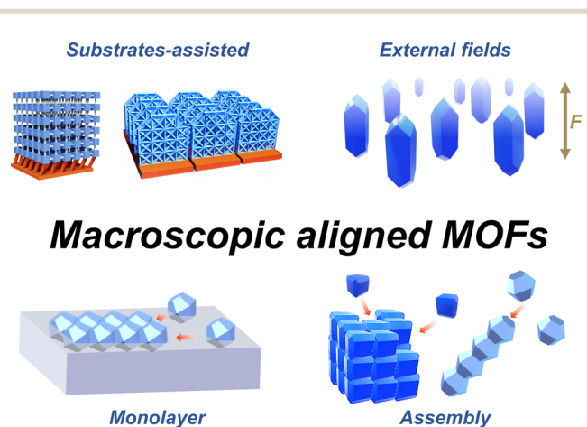
Fig. 1 Schematic illustration of a variety of methods for preparing macroscopic aligned MOFs.
