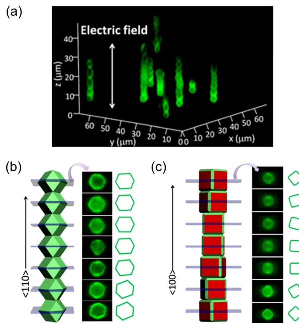
Fig. 13 (a) In situ confocal microscope observations of rhombic dodecahedral ZIF-8 particles assembled into a homogeneous 1D chain under the influence of a 1 MHz electric field. Scheme of 1D chains composed of (b) rhombic dodecahedral ZIF-8 particles with the (110) planes in contact and (c) truncated cubic ZIF-8 particles with the (100) planes in contact, along with confocal images of cross-sectional ZIF-8 particles within the 1D chains. Adapted with permission from ref. 95. Copyright 2013, American Chemical Society.
