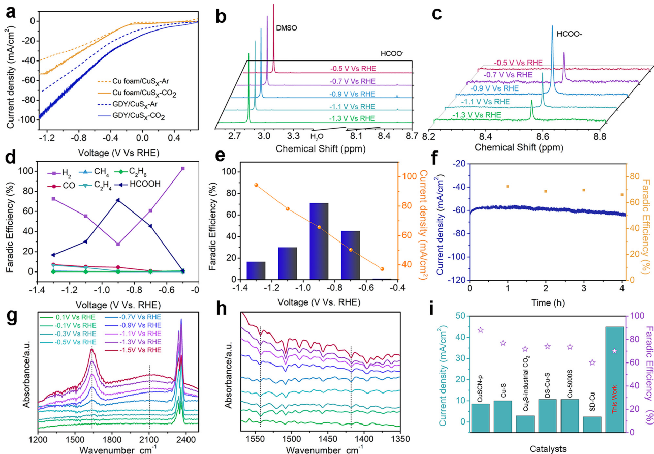
Fig. 4 (a) Linear sweep voltammetry of \text{CuS}_x and \text{GDY/CuS}_x recorded in \text{CO}_2^- and \text{Ar}^- saturated electrolytes. (b and c) ^1\text{H} NMR spectra of the electrolyte after the \text{CO}_2\text{RR} at the \text{GDY/CuS}_x electrode at different applied potentials. (d) Potential–faradaic efficiency (FE) curves for the products ( \text{HCOOH} , \text{H}_2 , \text{CO} , \text{C}_2\text{H}_4 , and \text{C}_2\text{H}_6 ) produced during the \text{CO}_2\text{RR} on \text{GDY/CuS}_x . (e) Plot of FE and current density of \text{GDY/CuS}_x vs. the potential. (f) Stability and the corresponding faradaic efficiency for \text{HCOOH} produced with \text{GDY/CuS}_x at -0.9 V vs. RHE in \text{CO}_2 -saturated 0.1 M \text{KHCO}_3 . (g and h) Potential-dependent in situ ATR-FTIR spectra of the \text{GDY/CuS}_x electrode with \text{CO}_2 purging. (i) Comparison between \text{GDY/CuS}_x and reported Cu-based electrodes for the \text{CO}_2\text{RR} .
