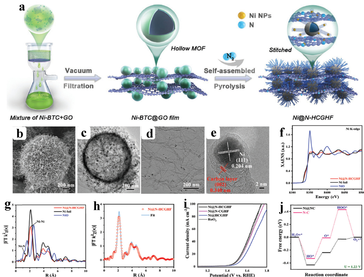
Fig. 11 (a) Schematic representation of Ni@N-HCGHF; (b) SEM and TEM images of N-doped MOF-derived carbon nanotube hollow microspheres; (c) HR-TEM images; (d–e) HR-TEM images of Ni@N-HCGHF; (f and g) Ni-K edge XANES spectra and FT-EXAFS spectra of Ni@N-HCGHF, Ni foil, and NiO; (h) EXAFS fitting curves of Ni@N-HCGHF; (i) LSV outcomes of Ni@N-HCGHF, Ni@N-CGHF, Ni@HCGHF and RuO 2 ; (j) calculated Gibbs free energy diagram of the OER intermediates of Ni@N-HCGHF. Reprinted with permission from ref. 81. Copyright (2020) Wiley-VCH.
