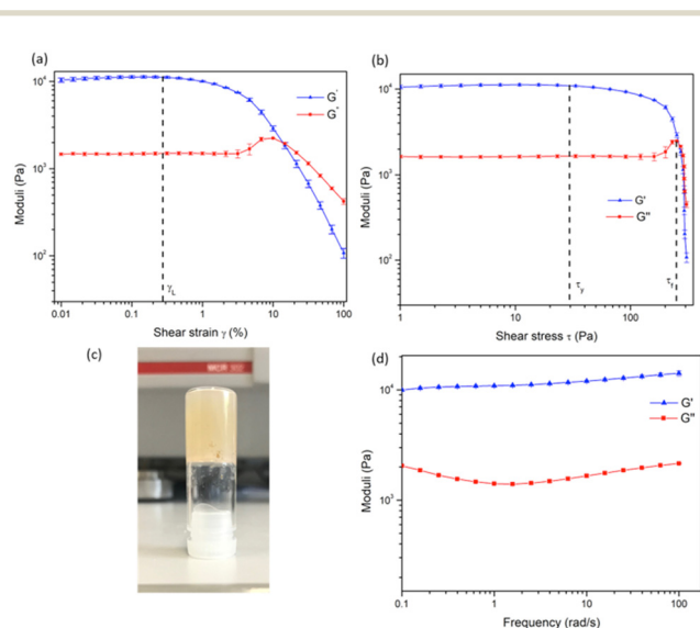
Fig. 5 (a) Amplitude (strain) sweep experiment of 1 gel showing the linear viscoelastic region ( \gamma_L ) and confirming the behaviour of the material as a gel. (b) Amplitude (stress) sweep showing yield point ( \tau_y ) and flow point ( \tau_f ) of the material. (c) Image of the gel during inversion test. (d) Frequency sweep experiment showing the long-term stability of the gel.
