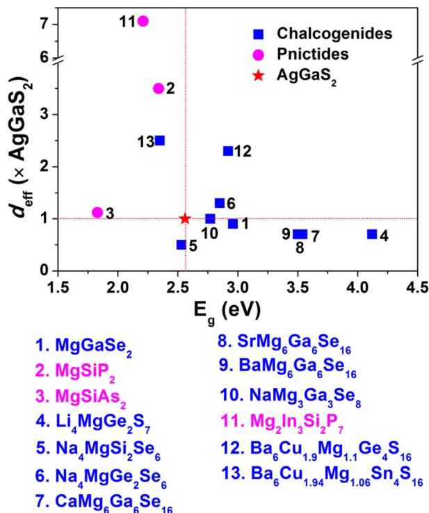
Fig. 15 Comparison of the d_{eff} ( \times AGS) and E_g (eV) for selected Mg-based materials with IR NLO properties.
