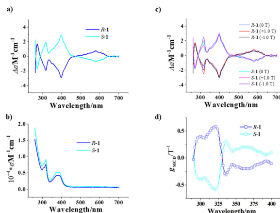
Fig. 5 CD spectra of R-1 and S-1 at room temperature (MeCN, c = 0.2 g L -1 , optical path = 1 mm) (a). UV-visible spectra of R-1 and S-1 at room temperature (MeCN, c = 0.2 g L -1 , optical path = 1 mm) (b). CD spectra in a MeCN solution at room temperature ( c = 0.2 g L -1 , optical path = 1 mm, H = 0 and \pm 1.0 T) (c). g_{\text{MCD}} of R-1 and S-1 (d).
