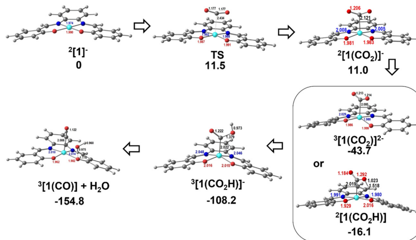
Fig. 10 Optimised structures of the intermediates in CO 2 binding to 2[1]^\bullet and reduction to CO: TS between 2[1]^\bullet and 2[1(\text{CO}_2)]^\bullet , 3[1(\text{CO}_2)]^{2-} or 2[1(\text{CO}_2\text{H})]^\bullet , 3[1(\text{CO}_2\text{H})]^\bullet , and 3[1(\text{CO})] + \text{H}_2\text{O} .
