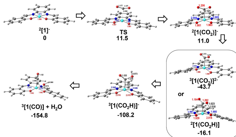
Fig. 10 Optimised structures of the intermediates in CO 2 binding to 2[1]^\bullet- and reduction to CO: TS between 2[1]^\bullet- and 2[1(\text{CO}_2)]^\bullet- , 3[1(\text{CO}_2)]^{2-} or 2[1(\text{CO}_2\text{H})] , 3[1(\text{CO}_2\text{H})]^\bullet- , and 3[1(\text{CO})] + \text{H}_2\text{O} .
