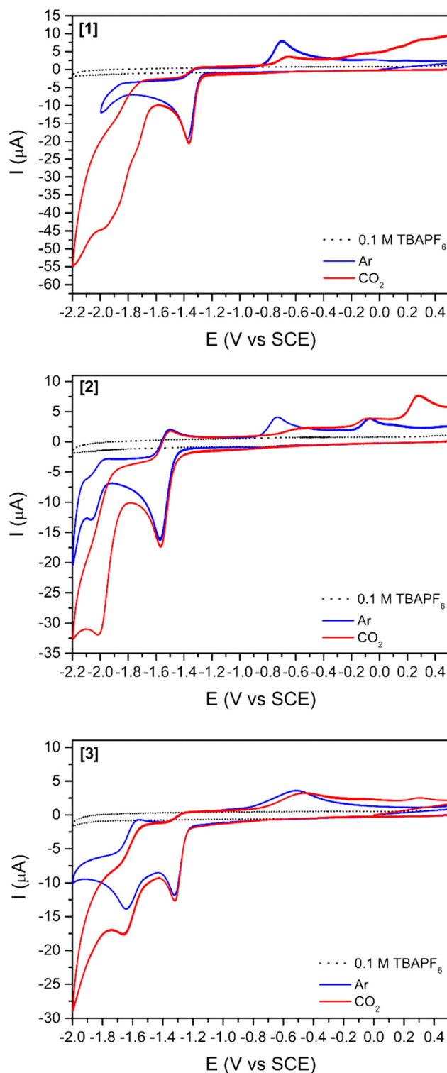
Fig. 2 Cyclic voltammograms of complexes [1], [2], and [3] (1 mM) in DMF, argon, or carbon dioxide saturated solutions using TBAPF 6 as supporting electrolyte (0.1 M) at 100 \text{ mV s}^{-1} . Glassy carbon (3 mm diameter) was used as working, platinum wire as counter and SCE as reference electrodes.
