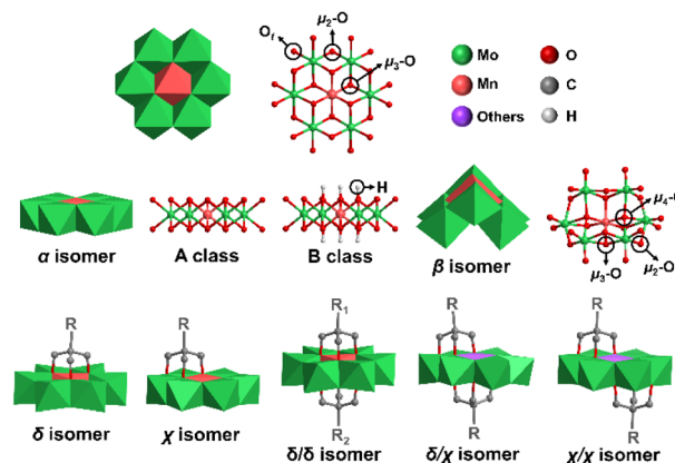
Fig. 1 Structures and isomeric species of Anderson-type POMs, and isomeric species after modification with triol ligands. Color code: {MoO 6 }, green octahedron; {MnO 6 }, red octahedron; {XO 6 }, violet octahedron (X = others). Hydrogen atoms in organic ligands have been omitted for clarity.
