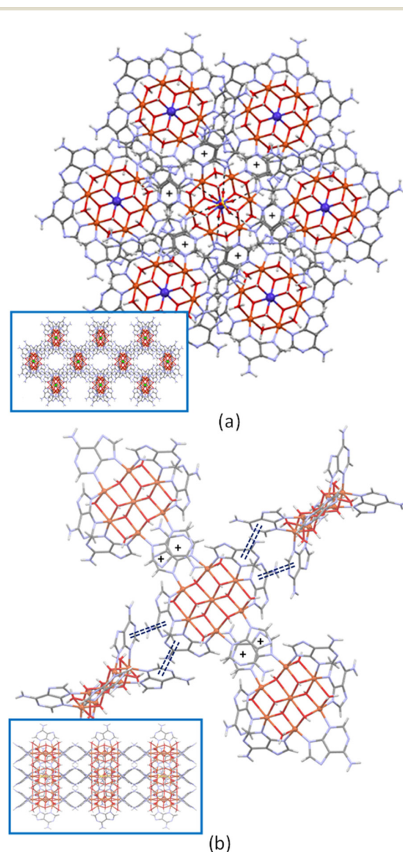
Fig. 2 Details of the \pi\text{-}\pi stacking interactions (+ symbol and double dashed lines) in compounds \text{Cu}_6\text{Zn} (a) and \text{Cu}_6\text{Cu} (b). The insets show a projection of the crystal packing.
