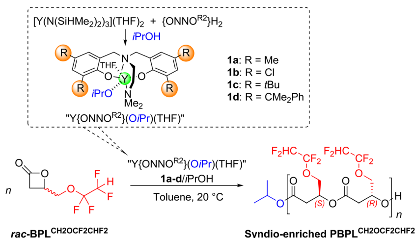
Scheme 3 Stereoselective ROP of racemic 4-((2,2,3,3-tetrafluoropropyl)methylene) β-propiolactone, rac -BPL CH 2 OCF 2 CHF 2 , catalyzed by diamino-bisphenolate yttrium complexes Y{ONNO R2 } 1a–d in the presence of i PrOH as the co-initiator.
