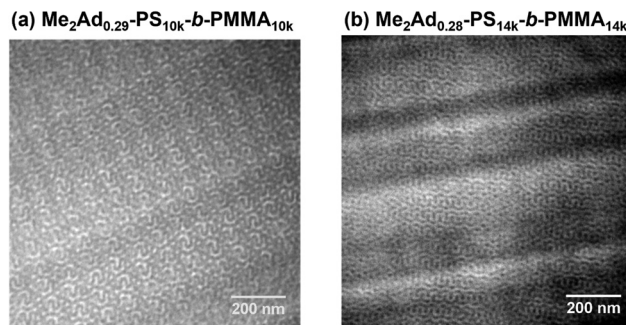
Fig. 9 TEM micrographs of (a) \text{Me}_2\text{Ad}_{0.29}\text{-PS}_{10k}\text{-}b\text{-PMMA}_{10k} (annealed at 200 °C for 24 h) and (b) \text{Me}_2\text{Ad}_{0.28}\text{-PS}_{14k}\text{-}b\text{-PMMA}_{14k} (annealed at 250 °C for 24 h).
