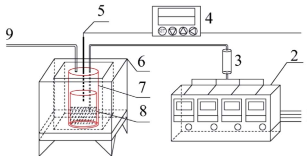
Fig. 1 Schematic diagram of the sample preparation device 1-gas source; 2-gas mass flow meter; 3-gas mixing tank; 4-program temperature controller; 5-K type thermocouple; 6-high temperature combustion furnace; 7-stainless steel tank; 8-corundum crucible; 9-gas outlet.
