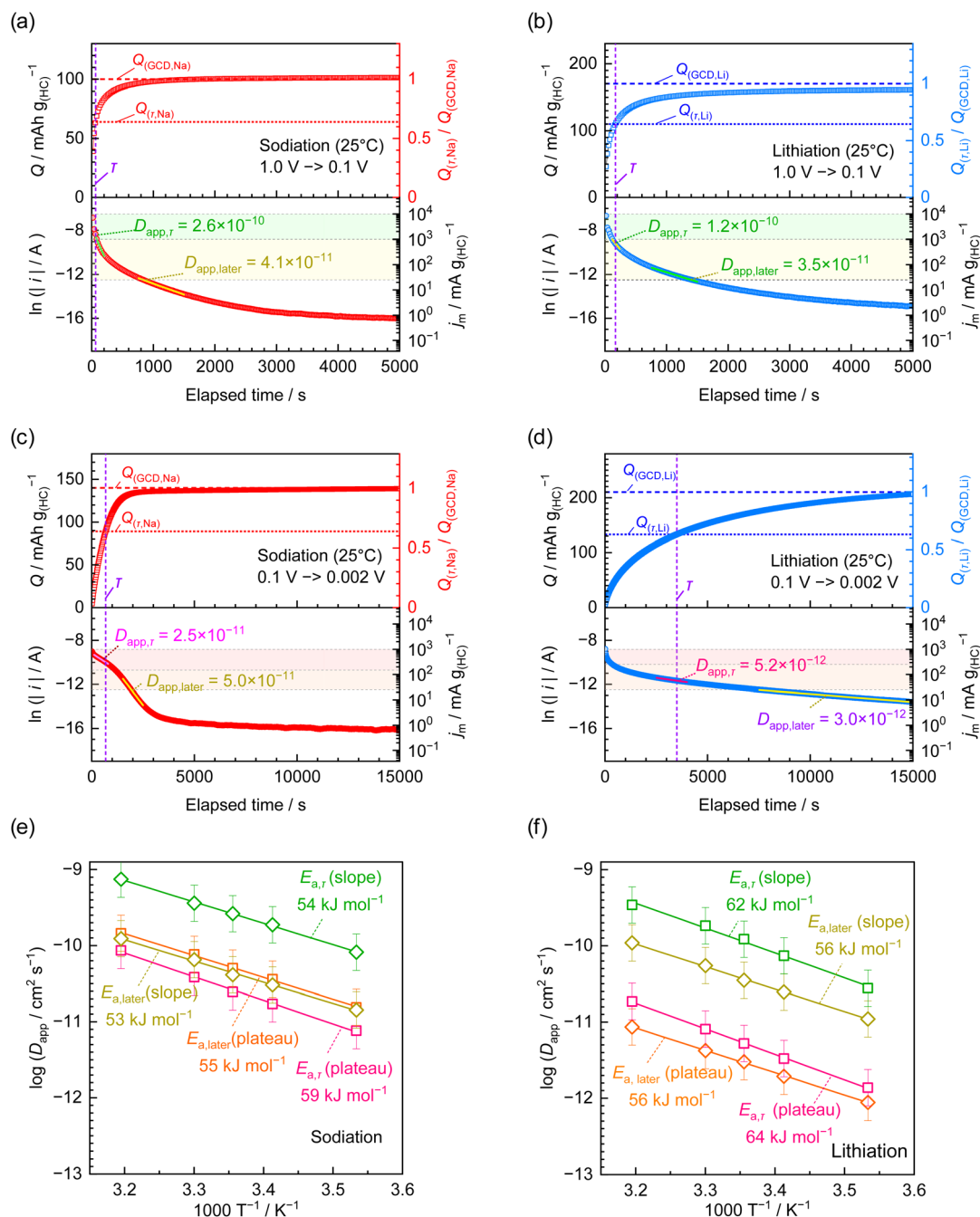
Fig. 6 Chronocoulougrams and corresponding chronoamperograms of 5 vol% HC electrodes for the slope regions of (a) sodiation and (b) lithiation and plateau regions of (c) sodiation and (d) lithiation. The values of D_{\text{app}} were estimated by applying eqn (4), as described in the Experimental section. Activation energies E_{a,\tau} and E_{a,\text{later}} were estimated from D_{\text{app}} vs. T^{-1} plots of D_{\text{app},\tau} and D_{\text{app},\text{later}} during (e) sodiation and (f) lithiation, respectively. The error bars of D_{\text{app}} values are estimated from standard error of the HC particle size.
