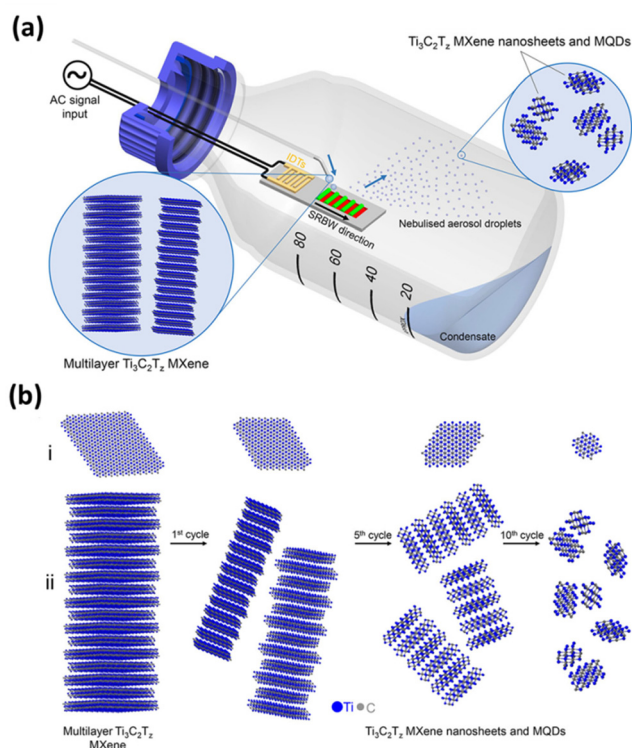
Fig. 2 (a) Schematic illustration of the experimental setup for the acoustofluidic synthesis of pristine ultrathin \text{Ti}_3\text{C}_2\text{T}_z MXene nanosheets and MQDs. Here, the multilayer \text{Ti}_3\text{C}_2\text{T}_z MXene sample is continuously delivered to the SRBW device. The delaminated and cleaved \text{Ti}_3\text{C}_2\text{T}_z condenses within the glass bottle enclosure after forming the aerosol droplets in the top by nebulization. (b) The condensate collected after many cycles at the bottom undergoes successive renebulization to form (i) laterally cleave and (ii) delaminate the sample into smaller and thinner MXene nanosheets and MQDs. Reproduced with permission from ref. 68. Copyright © 2021, American Chemical Society.
