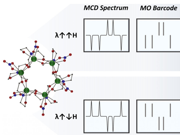
Scheme 1 (Left) Crystal structure of [\text{Er}_6(\text{teaH})_6(\text{NO}_3)_6] \cdot 6\text{Er}_3 (colour code: green (Er); red (O), blue (N), black (C)) MCA (CCDC number: 1876163). (Right) representation of the dual-signalled magneto-optical barcode obtained via MCD spectroscopy.
