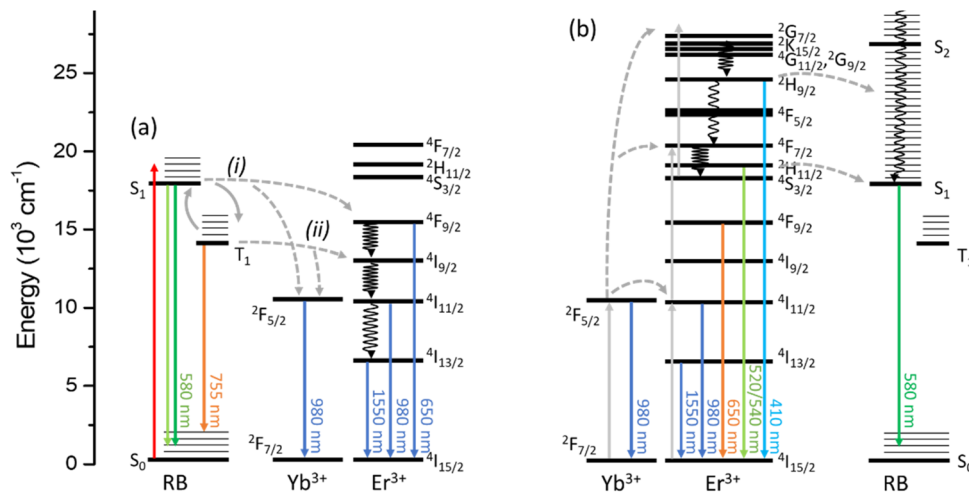
Fig. 1 Energy diagram of photophysical processes observed for \text{UC}_{\text{Er}}\text{@RB} under \text{N}_2 exciting the (a) dye ( \lambda_{\text{exc}} = 560 \text{ nm} ) or the (b) UCNP ( \lambda_{\text{exc}} = 980 \text{ nm} ).
