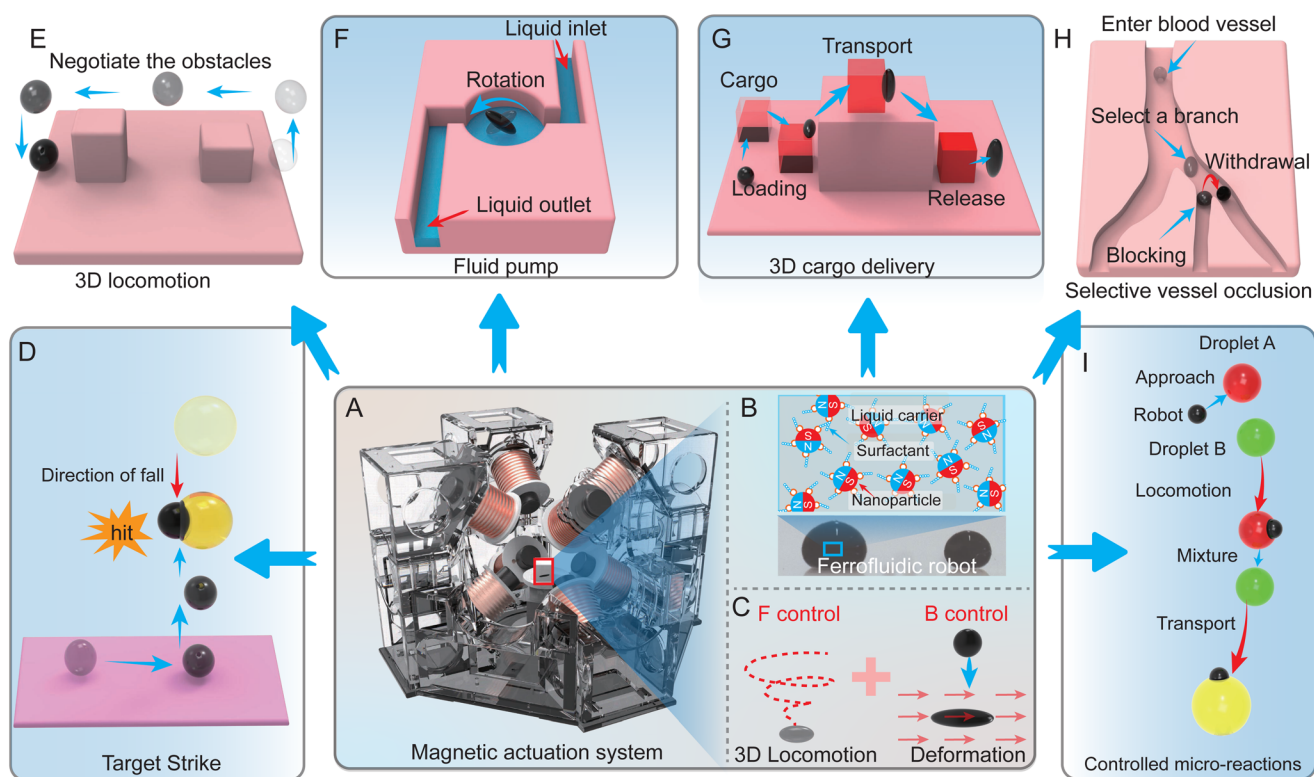
Fig. 1 Exploring magnetic drive systems and their varied experimental applications. (A) An illustration of an eight-axis magnetic control system, depicting the comprehensive design that enables the intricate control of magnetic fields. (B) A conceptual diagram that provides insight into the complex composition of ferrofluids, detailing their unique properties. (C) A visual demonstration illustrating how force influences the trajectory of the robot and how torque controls its directional orientation. (D) A conceptual representation of a ferrofluidic robot for interception, detailing how robots interact with surrounding invaders. (E) A schematic outlining the concept of complex path obstacle avoidance, illustrating how the robot negotiates around obstacles. (F) A conceptual diagram of a fluid pumping experiment, demonstrating the utility of the ferrofluidic robot in micro-pump applications. (G) A diagram visualizing a 3D transport experiment, exemplifying the robot's capability to move in all three spatial dimensions. (H) A conceptual illustration of selective vascular occlusion, demonstrating the potential use of the robot in targeted medical interventions. (I) A diagram showcasing a droplet mixing experiment, exemplifying the robot's ability in micro-scale mixing applications.
