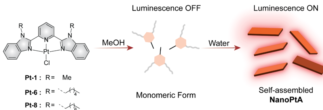
Scheme 1 A schematic illustration of NanoPtA assembly formation in water with variation in chain length resulting in different luminescence.
