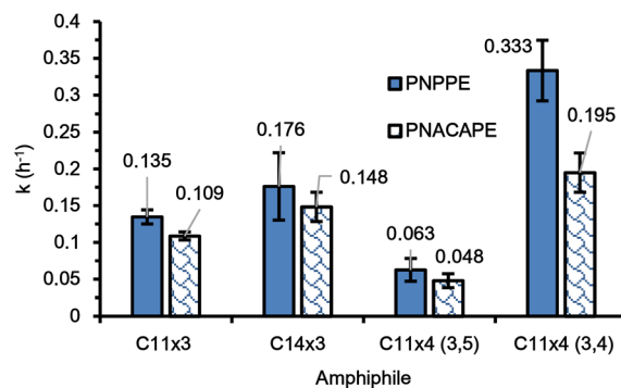
Fig. 5 Rate constants of PNPPE (blue, solid fill) and PNACAPE (blue, shingle pattern) depropargylation in presence of C11×3, C14×3, C11×4 (3,5) and C11×4 (3,4) metallic micelles.
