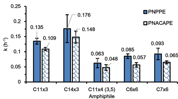
Fig. 4 Rate constants of PNPPE (blue, solid fill) and PNACAPE (blue, shingle pattern) depropargylation in presence of C11×3, C14×3, C11×4 (3,5), C6×6 and C7×6 metallic micelles.
