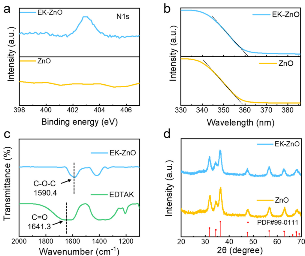
Fig. 1 (a) XPS spectra of N 1s, (b) UV-vis absorption spectra, (c) FTIR spectra and (d) XRD patterns of ZnO and EK-ZnO films.
