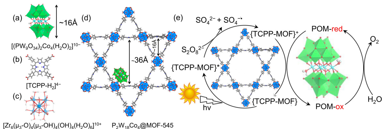
Fig. 5 POM@MOF-545 components: (a) \text{P}_2\text{W}_{18}\text{Co}_4 POM; (b) TCPP- \text{H}_2 linker; (c) Zr-based unit; and (d) \text{P}_2\text{W}_{18}\text{Co}_4@ MOF-545. The position of the POM is obtained from computations. \text{WO}_6 , green polyhedra; \text{ZrO}_8 , blue polyhedra or spheres; Co, cyan spheres; O, red spheres; C and H, gray; N, dark blue. (e) Schematic representation of the proposed mechanism for the light-driven OER by \text{P}_2\text{W}_{18}\text{Co}_4@ MOF-545. Adapted with permission from ref. 80. Copyright 2018, American Chemical Society.
