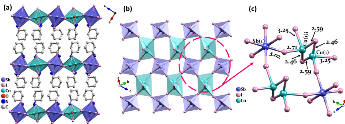
Fig. 1 (a) The crystal structure of the 2D layered double perovskite CuSbI-1 (hydrogen atoms are omitted for clarity). (b) The platform of 2D inorganic layers consisting of alternating \text{Cu-I}_6 octahedrons and \text{Sb-I}_6 octahedrons. (c) The framework of the \text{Cu-I-Sb} octahedrons with different \text{Cu-I} and \text{Sb-I} bond lengths. (i): x, y - 1, z .
