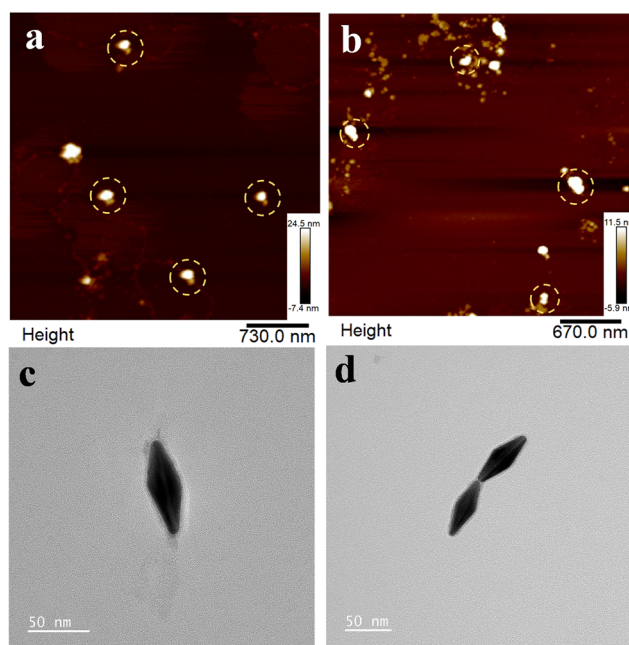
Fig. 2 AFM images of Au NBPs: (a) monomer and (b) dimer, and TEM images of Au NBPs: (c) monomer and (d) dimer.
