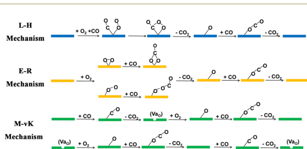
Scheme 1 Three different mechanisms of COOR catalysis.
