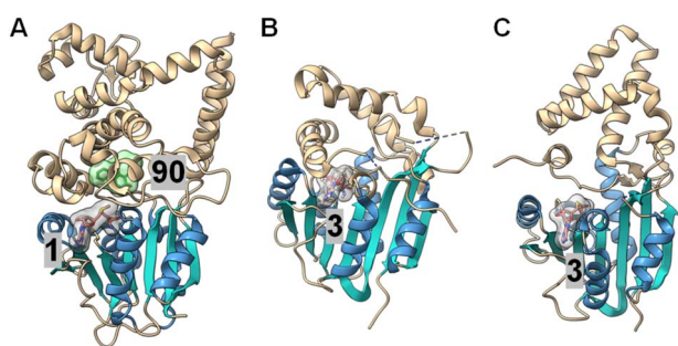
Fig. 21 Crystal structures of (A) LepI (PDB ID: 6IX5), (B) SpnF (PDB ID: 4PNF) and (C) SpnL (PDB ID: 7V6H). Each enzyme contains a C-terminal Rossmann fold catalytic domain containing seven \beta -strands (cyan) surrounded by five \alpha -helices (blue), while the N-terminal domains differ between each protein. The cofactor, SAM ( 1 ) for LepI and SAH ( 3 ) for SpnF and SpnL (pink with a gray surface), binds similarly at the C-terminal domain of all three enzymes. The substrate analog ( 90 ) bound in the LepI active site is shown with a green surface.
