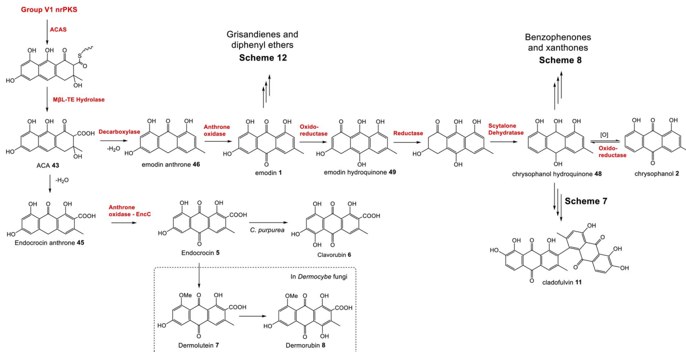
Scheme 2 The core biosynthetic pathway of the emodin family of natural products proceeds via atrochryson carboxylic acid (ACA) 43 , the anthraquinones emodin 1 and chrysophanol 2 , and their corresponding hydroquinones.
