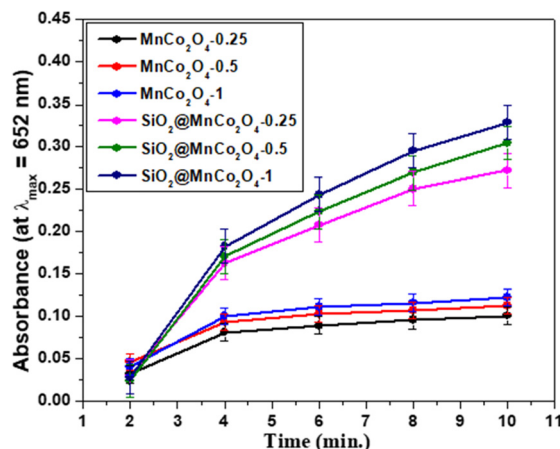
Fig. 7 Peroxidase-like activity of \text{MnCo}_2\text{O}_4 NPs and \text{SiO}_2@\text{MnCo}_2\text{O}_4 core-shell nanorattles as indicated by time dependent absorbance.
