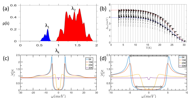
Fig. 4 EPC strength distribution, superconducting gap and DOS of \text{LaB}_2 (a) EPC distribution \rho_{nk} as a function of the EPC strength \lambda_{nk} . (b) Superconductivity gap distribution at the Fermi surface from T = 3 K to T = 30 K. Blue and red dash curves are obtained from fitting the superconductivity gap equation using the maximum gap distribution. (c) Quasiparticle density of states at T = 5 K, 15 K, 25 K, 30 K (blue, red, yellow, and purple curves, respectively). (d) Zoom in plot of (c). Gray arrows indicate the 2 gaps.
