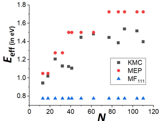
Fig. 9 Comparison of E_{\text{eff}} for closed-shell Ag TP from KMC simulation, beyond-MF MEP analysis, and refined-MF analysis for a ranges of sizes, N .
