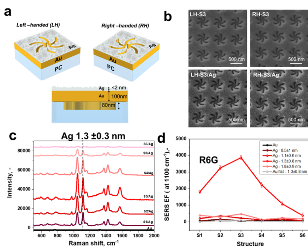
Fig. 1 (a) Schematic description of plasmon-active SERS substrates with coupled chiral active shuriken and cluster-like Ag layer; (b) SEM images of LH- and RH-handled shuriken structures before and after Ag deposition; (c) SERS spectra of R6G, measured at 785 nm on RH-S x /Ag structures as a function of shurikens geometry; (d) dependence of SERS enhancement factors on shurikens geometry and silver effective thickness.
