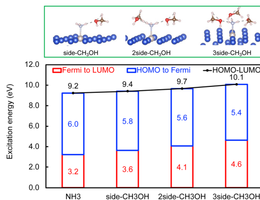
Fig. 3 The effect of CH 3 OH on interfacial charge and energy transfer. The energy to excite an electron from the HOMO of NH 3 to the Fermi level (blue), from the Fermi level to the LUMO of NH 3 (red), and from the HOMO to the LUMO (black). Optimized configurations of NH 3 with CH 3 OH on RuCu 83 are shown in the top panel.
