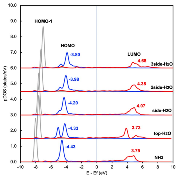
Fig. 2 Density of states projected onto frontier orbitals of NH 3 adsorbed on RuCu 83 with and without water. The center of the HOMO and LUMO of NH 3 are shown above the main peak.
