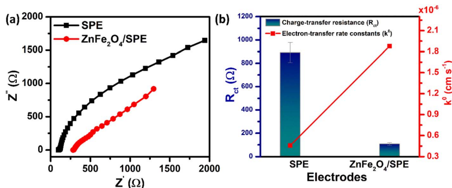
Fig. 3 (a) EIS plots in 5 mM [\text{Fe}(\text{CN})_6]^{3-/4-} solution containing 0.1 M KCl for the unmodified and \text{ZnFe}_2\text{O}_4 -modified SPE; (b) the bar chart diagram of the charge-transfer resistance ( R_{\text{ct}} ) and the heterogeneous electron-transfer rate constant ( k^0 ) value of the bare SPE and \text{ZnFe}_2\text{O}_4/\text{SPE} .
