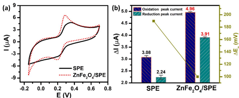
Fig. 4 (a) CV curves and (b) the bar diagram of redox peak currents of 50 \mu\text{M} PCM in 0.1 M PBS (pH 5.0). The scan rate of CV is 70 \text{mV s}^{-1} .
