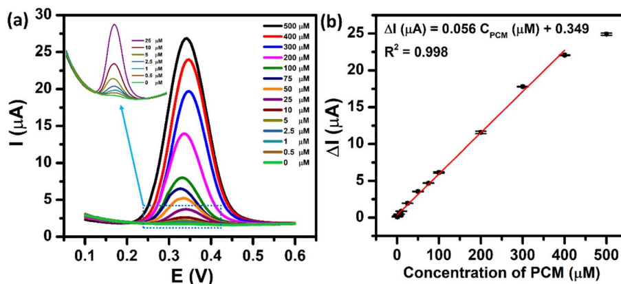
Fig. 9 (a) DPV curves of 0–500 μM PCM in 0.1 M PBS (pH 5.0) at the ZnFe 2 O 4 /SPE and (b) the calibration plots of oxidation peak current responses vs. various concentrations of PCM with error bars.
