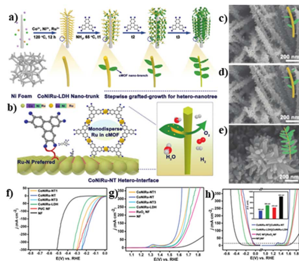
Fig. 4 (a and b) Illustration of the design of cMOF/LDH hetero-nano-tree catalysts for overall water splitting; (c–e) SEM images of CoNiRu-NT 1–3; LSV curves of (f) HER, (g) OER and (h) water splitting; (h-inset) the value of \Delta E of different catalysts. Reproduced with permission from ref. 64. © Wiley-VCH GmbH, 2022.
