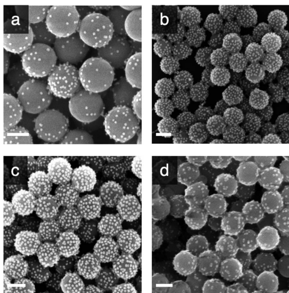
Fig. 2 Representative scanning electron micrographs of SPs, reacted with increasing concentrations of APTES [2.6 (a), 7.8 (b) and 26 (c) mM] and reacted with AuNPs at a concentration of 0.310 mg mL -1 . In (d), are shown SPs reacted with 26 mM of AuNPs and with glutaraldehyde (0.1%, v/v). All scale bars represent 200 nm.
