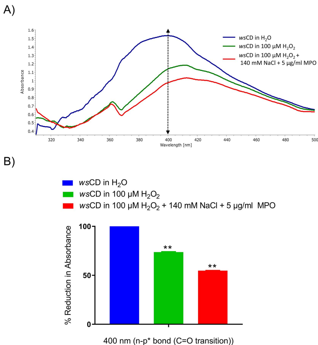
Fig. 9 Enzymatic biodegradation of wsCDs. (A) UVB absorption spectra (300–500 nm) of wsCDs treated with H 2 O, 100 \mu\text{M H}_2\text{O}_2 , and a complete peroxide system, (5 \mu\text{g ml}^{-1} human origin MPO, 140 mM NaCl, and 100 \mu\text{M H}_2\text{O}_2 ) for 24 h; (B) UV absorbance of wsCDs suspended under various conditions at 400 nm. The results represent mean \pm SD. Statistical analysis through one-way ANOVA followed by Tukey's post hoc test. ** p -value < 0.01 (treatments vs. H 2 O suspension).
