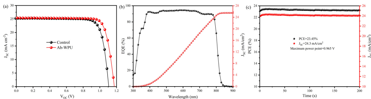
Fig. 4 (a) J - V curve of the best device of perovskite solar cell without additives and modified by AB-WPU, (b) EQE spectrum and integrated current density, and (c) MPP stable power output.
