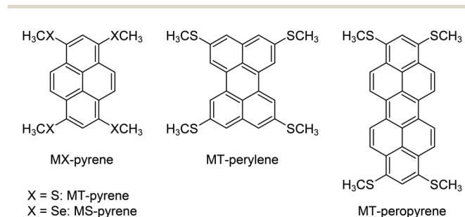
Fig. 1 Molecular structures of 1,3,6,8-tetrakis(methylthio)- and 1,3,6,8-tetrakis(methylseleno)-pyrene and (MT- and MS-pyrene), 2,5,8,11-tetrakis(methylthio)ptylene (MT-ptylene), and 1,3,8,10-tetrakis(methylthio)peropyrene (MT-peropyrene).
