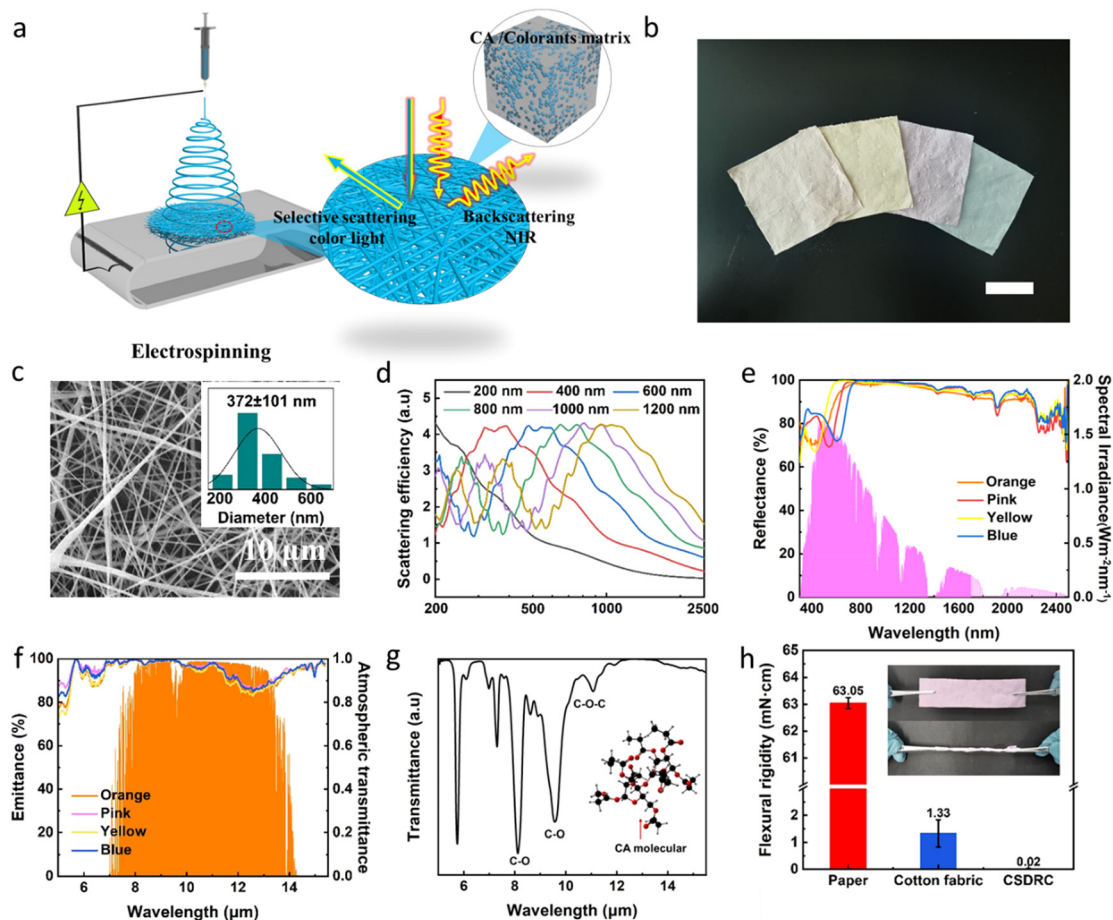
Fig. 2 (a) Schematic illustration of the preparation of CA NF CSDRC. (b) Photograph of CA NF CSDRCs with different colors. The thickness of the film is 500 \mu m. Scale bar, 5 cm. (c) SEM images of CSDRCs with different colors, insets: the diameter distribution of the corresponding image. (d) The calculated scattering efficiency of CA NF in the solar region. (e) The optical reflectance of CA NF CSDRCs in the solar region. AM1.5 solar spectrum was depicted as a reference. (f) Optical emittance of the CA NF CSDRCs in the MIR region. Atmospheric transmittance was acquired by simulation (Modtran) and depicted as a reference. (g) The IR transmittance of the CA NF CSDRCs in the MIR region. (h) The flexural rigidity comparison of printing paper, cotton fabric and CA NF CSDRC, inset shows the twisted flexible film.
