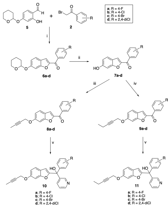
Scheme 2 Synthesis of 6- O -but-2-ynyl ( 10 ) and 6- O -pent-2-ynyl ( 11 ) compounds. Reagents and conditions: (i) K_2CO_3 , CH_3CN , 70\text{ }^\circ C , 3 h, 52–86%; (ii) HCl , dioxane, rt, 1 h 64–71%; (iii) K_2CO_3 , CH_3CN , 40\text{ }^\circ C , 1 h, then 1-bromobut-2-yne, rt, 16 h, 34–86%; (iv) K_2CO_3 , CH_3CN , 40\text{ }^\circ C , 1 h, then 1-bromopent-2-yne, rt, 16 h, 35–76%; (v) pyridine 3-magnesium bromide (prepared in situ ), THF, 70\text{ }^\circ C , 16 h, 10 34–90%, 11 15–91%.
