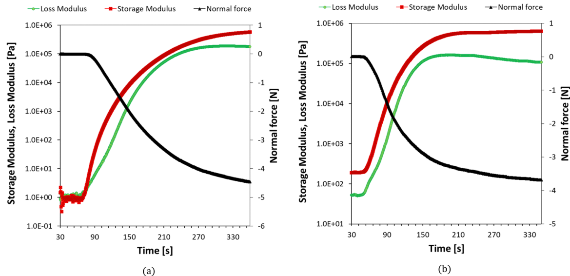
Fig. 14 (a) The storage (red) and loss modulus (green) as well as normal force (black) as a function of the illumination time for SPOT LV nanoresin: Ebecryl ® 4858/IBOA (0.7/0.3 w/w) + IOD (3.0 wt%)/NS (0.1 wt%) + 5% of Ag 2 O. (b) The storage (red) and loss modulus (green) as well as normal force (black) as a function of the illumination time for SPOT LV nanoresin: Ebecryl ® 4858/IBOA (0.7/0.3 w/w) + IOD (3.0 wt%)/NS (0.1 wt%) + 10% of HA. Film thickness 100 \mu\text{m} , irradiation power 4.8 \text{mW cm}^{-2} (405 nm), dark period: 60 s.
