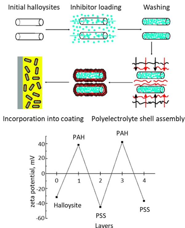
Fig. 2 Synthesis nanocarriers from halloysite loaded with 2-mercaptobenzothiazole. Zeta potential during polyelectrolyte deposition on halloysite nanotubes at pH 7.5. Reproduced from ref. 101 with permission of publisher. Copyright 2008 American Chemical Society.
