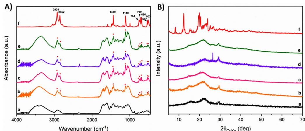
Fig. 3 FTIR (A) and WAXD (B) of B1 (a), B1/DTTP in a weight ratio of 1/0.5 (b), 1/1 (c), 1/2 (d) 1/3 (e) and DTPPBr (f).
