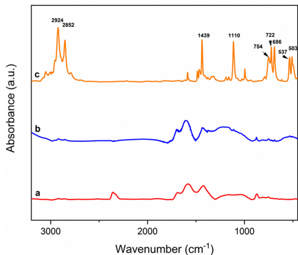
Fig. 8 FTIR spectra of (a) B2, (b) B2 after reaction with DTPP, and (c) DTPPBr.
