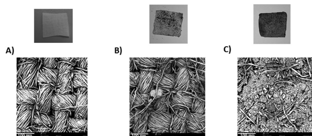
Fig. 9 Pictures and SEM images of (A) cotton fabric, (B) COTTON-B1, and (C) COTTON-B1/DTPP.
