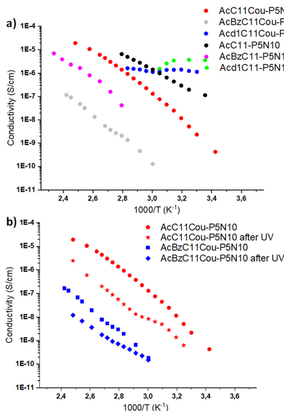
Fig. 5 (a) Conductivity variation with temperature, measured by EIS, of (a) all ionic compounds measured (b) AcC 11 Cou-P5N10 and AcBzC 11 Cou-P5N10 before and after irradiation with 325 nm light.
