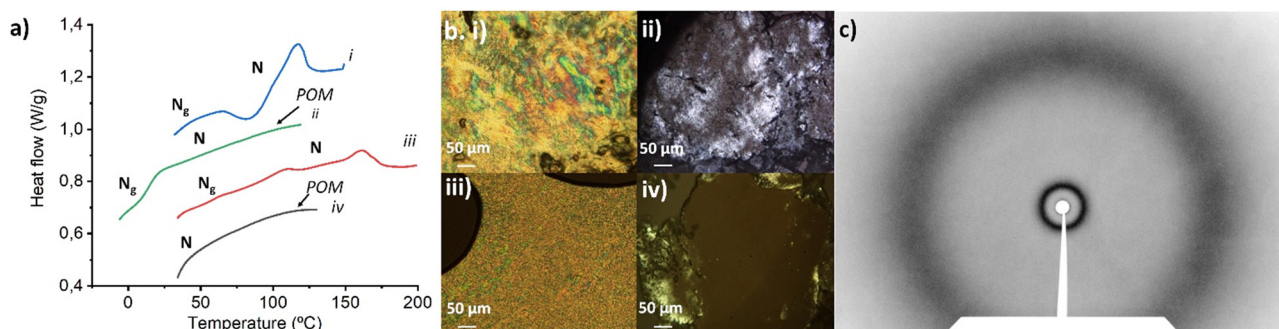
Fig. 4 (a) DSC curves in the second heating of (i) AcBzC 11 Cou-P5N10 (ii) Acd 1 C 11 Cou-P5N10 , (iii) AcBzC 11 -P5N10 and (iv) Acd 1 C 11 -P5N10 (b) POM textures of (i) AcBzC 11 Cou-P5N10 (ii) Acd 1 C 11 Cou-P5N10 , (iii) AcBzC 11 -P5N10 and (iv) Acd 1 C 11 -P5N10 (c) XRD example of AcBzC 11 Cou-P5N10 .
