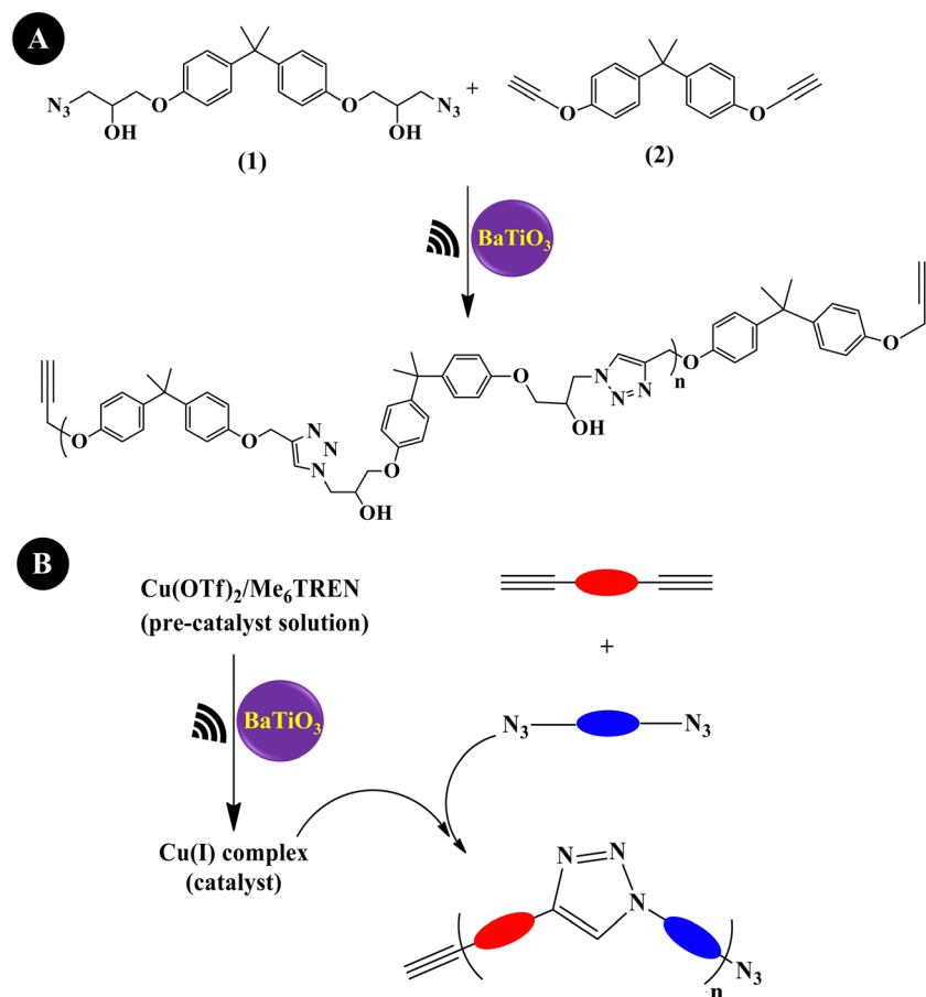
Fig. 8 Piezoelectrically mediated copper 'Click' polymerization of monomer 1 and monomer 2 (A) and a general depiction of Cu(I)-catalyzed Click polymerization (B) (adapted from ref. 204 with permission from Johns Wiley and Sons).
