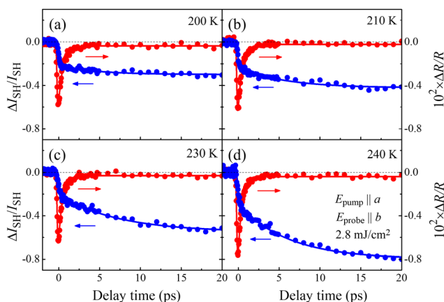
Fig. 4 (a)–(d) Time dependence of relative change of SHG ( \Delta I_{\text{SH}}/I_{\text{SH}} , blue circles) and reflectivity at 800 nm ( \Delta R/R , red circles) after the excitation by a pump pulse. The blue and red lines denote fitting results assuming a single exponential decay. (See text).
