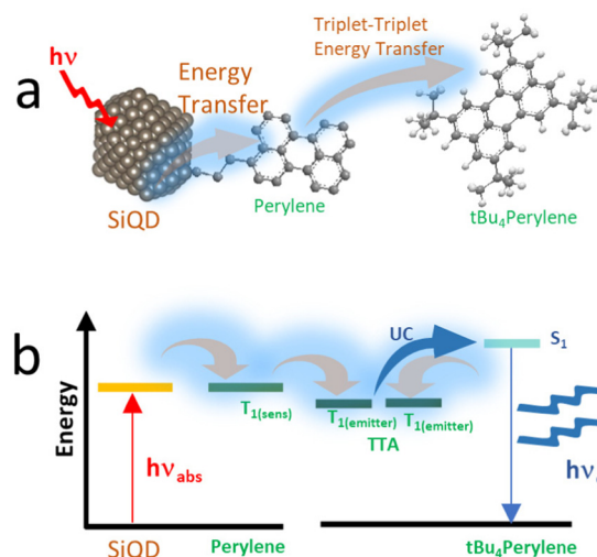
Fig. 12 (a) Triplet–triplet annihilation process of Perylene-functionalized SiQDs. (b) Triplet–triplet annihilation upconversion schematics by dye functionalized SiQDs immersed in the dye solvents. Adapted with permission from ref. 153. Copyright (2021) Royal Society of Chemistry.
