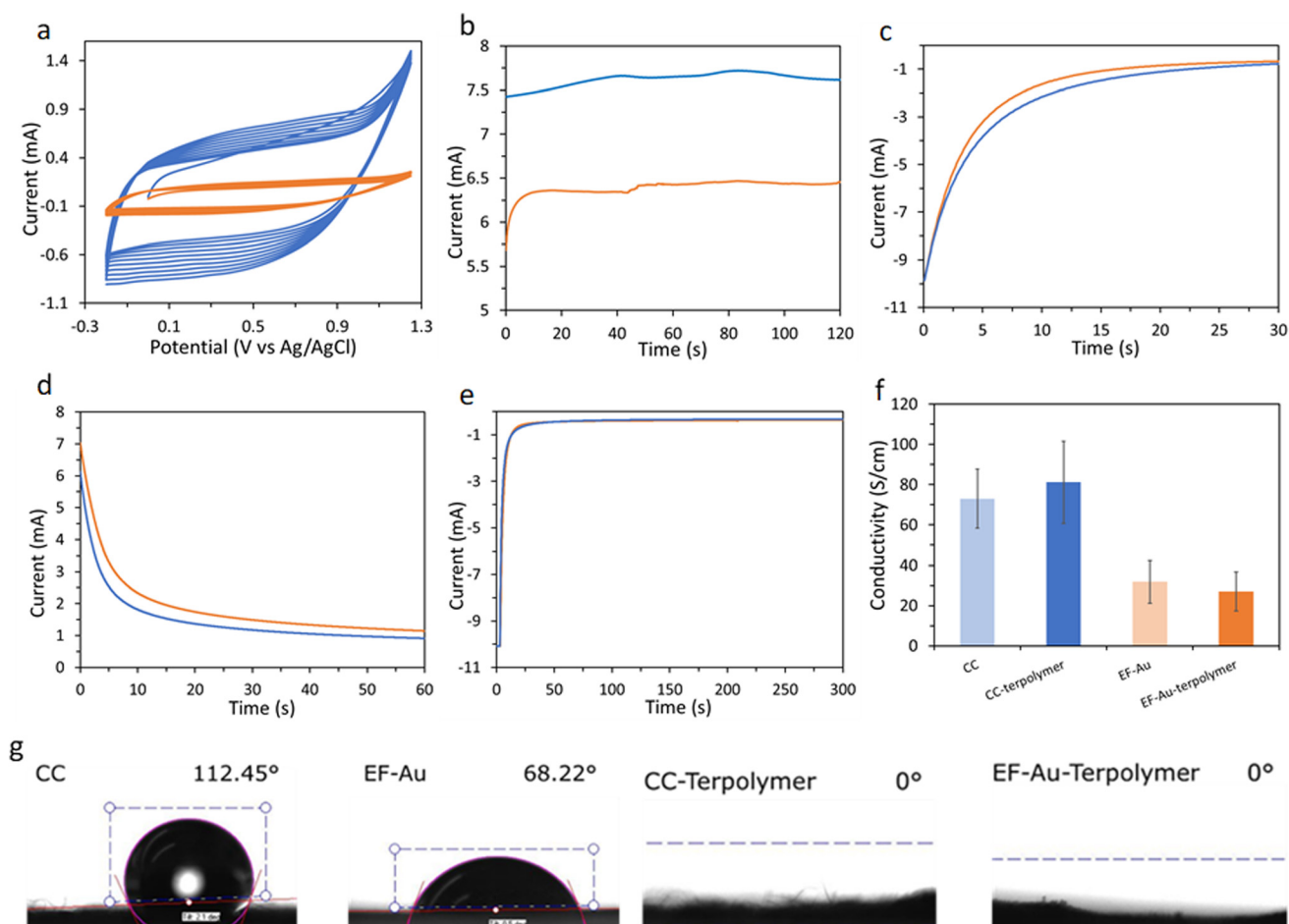
Fig. 2 (a) Potentiodynamic electropolymerization of P(EDOT- co -EDOTSac- co -EDOTEG) on carbon cloth (CC) (blue line) and PCL electrospun fibers (EF) (orange line) in 0.1 M LiClO 4 in water:acetonitrile (1:1 vol:vol) at 100 \text{ mV s}^{-1} , in the potential range from -0.2 to +1.25 V. (b–e) Chronoamperograms of carbon cloth (CC) (blue line) and PCL electrospun fibers (EF) (orange line): (b) the electropolymerization of the terpolymer P(EDOT- co -EDOTSac- co -EDOTEG) at +1.5 V ( vs. Ag/AgCl) for 2 min. (c) electrochemical reduction of P(EDOT- co -EDOTSac- co -EDOTEG) at a potential of -0.8 V ( vs. Ag/AgCl) for 30 seconds, (d) Conjugations of thiolated-ODN to the P(EDOT- co -EDOTSH- co -EDOTEG) at the potential of +1.0 V ( vs. Ag/AgCl) for 60 s. (e) chronoamperograms of the electrochemical release of ODN at -0.8 V ( vs. Ag/AgCl) for 5 min. (f) Electrical conductivity of the CC and the gold-coated EF mats before and after electrodeposition of P(EDOT- co -EDOTSac- co -EDOTEG) (g) Water contact angle measurements on CC and gold-coated EF before and after electrodeposition of P(EDOT- co -EDOTSac- co -EDOTEG).
