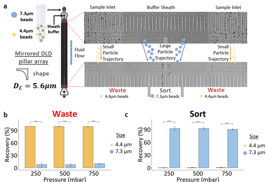
Fig. 2 Characterization of DLD sorting device. (a) Sorting characterization of the DLD device using 4.4 μm and 7.3 μm beads. The mirrored DLD device consists of an input region which has a central sheath buffer flow sandwiched by two sample co-flow streams. The outlet region of the DLD device shows the sorted region with two side waste channels which is characterized by the 4.4 μm and 7.3 μm beads shown in the waste and outlet (sort) region, respectively. (b) Graph showing the bead recovery in both the waste channels. (c) Graph showing the bead recovery in the sort channel. Paired two-tailed Student t -test was used to determine the statistical differences between outputs. **** denotes p value < 0.0001 for n = 4 samples.
